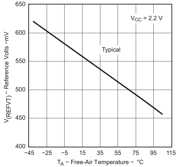
Figure 19. V (REFVT) vs Temperature, V CC = 2.2 V
